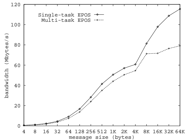
Fig. 5. Send bandwidth in EPOS.
