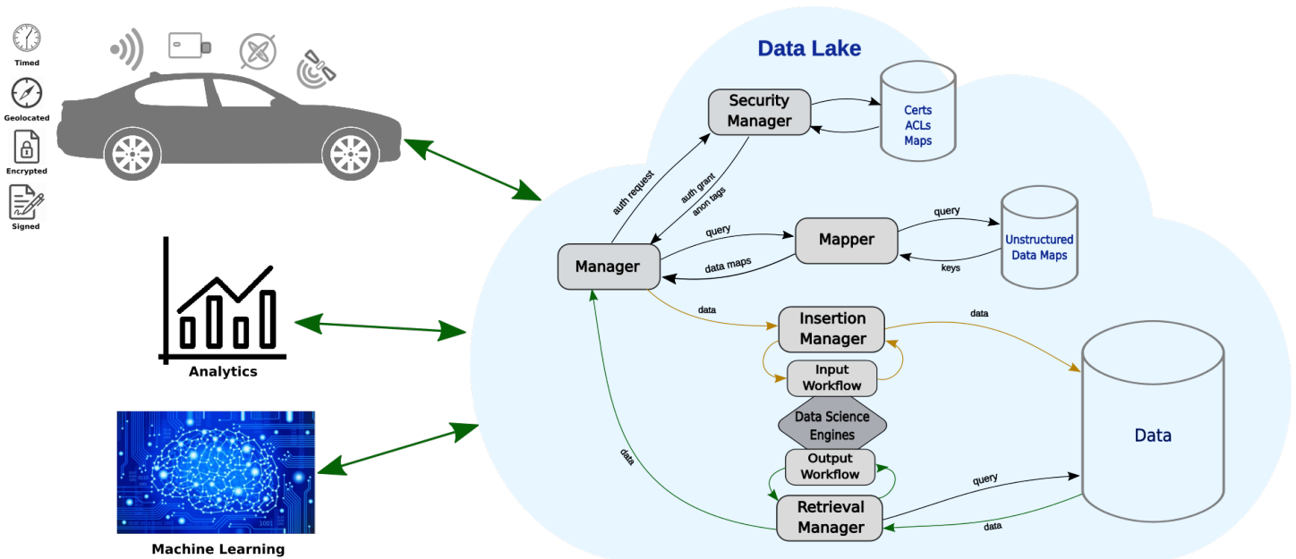
Fig 1: AutoDL Architecture Overview.
